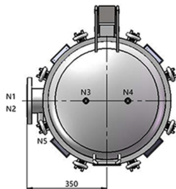
Nozzle Orientation
