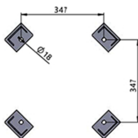
Leg Arrangement drawing
