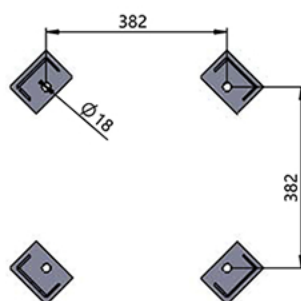
Leg Arrangement drawing
