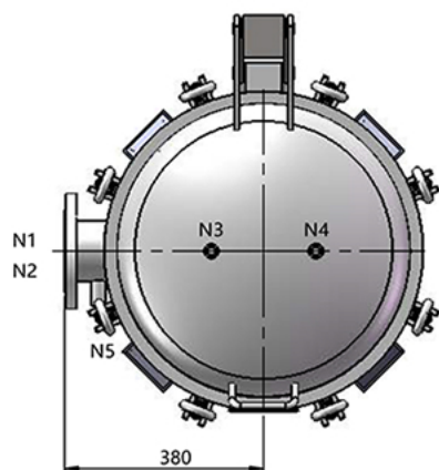
Nozzle Orientation
