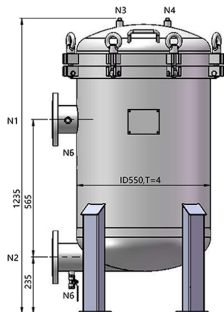
Nozzle Orientation
