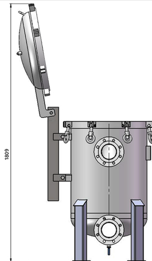
Leg Arrangement drawing
