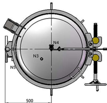
Nozzle Orientation
