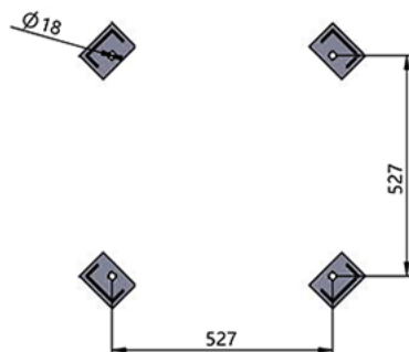
Leg Arrangement drawing
