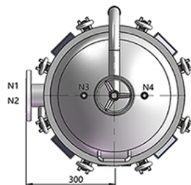
Nozzle Orientation
