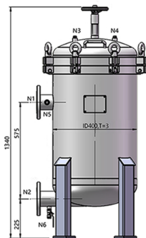
Nozzle Orientation
