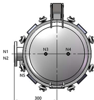
Nozzle Orientation
