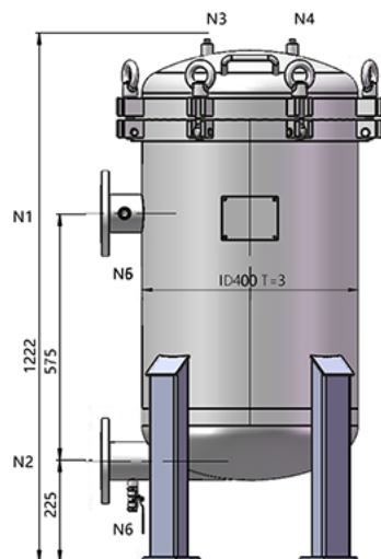
Nozzle Orientation
