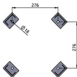
Leg Arrangement drawing
