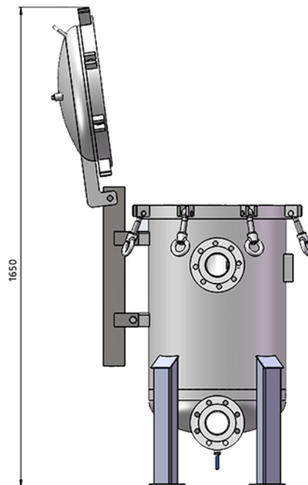
Leg Arrangement drawing
