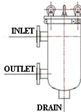
CF 3 side-in, same side-out
