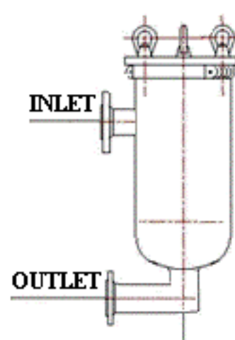
CF 7 side-in, same side bottom elbow-out
