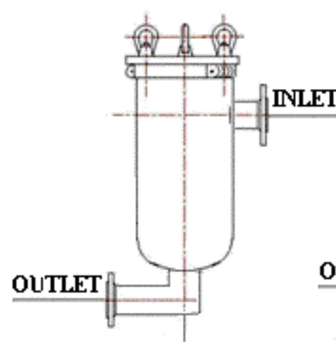
CF 8 side-in, bottom elbow-out
