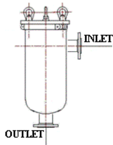
CF 1 side-in, bottom-out
