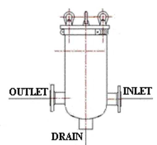
CF 10 side-in, side-out, inline for cartridge vessel only
